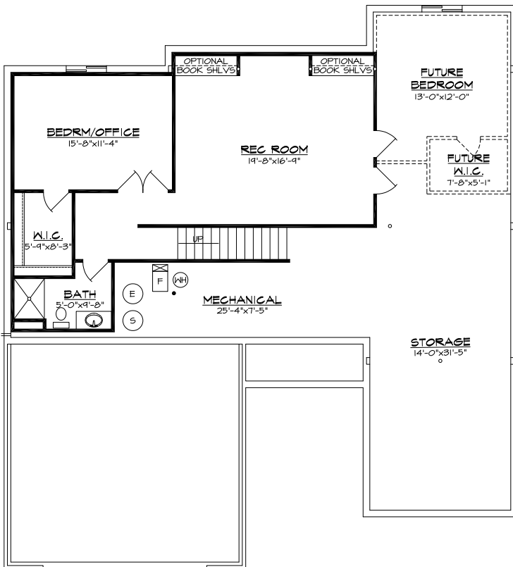
BASEMENT PLAN
